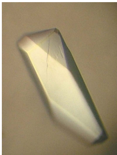
Figure 1 Crystal of L. interrogans DDG aldolase grown by the hanging-drop method.
